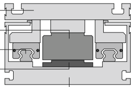
Herkömmliche Linearmotorachse Conventional linear motor module
